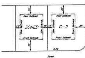
TYPICAL BUILDING SETBACK DETAIL 425
