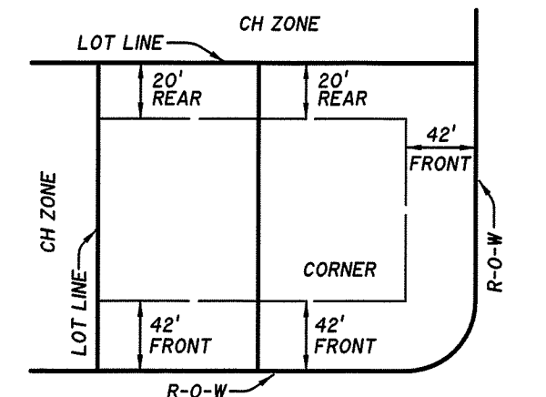
TYPICAL MINIMUM BUILDING SETBACKS FOR CH ZONING N.T.S.
